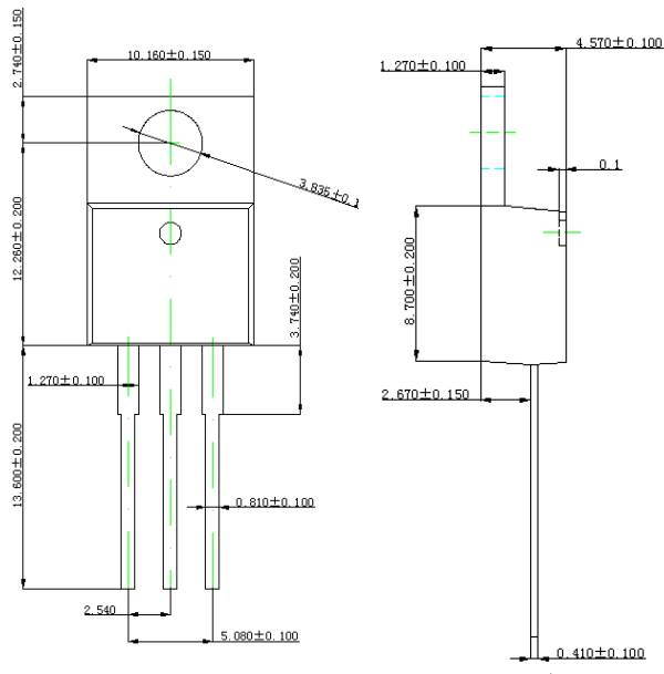
TO-220
