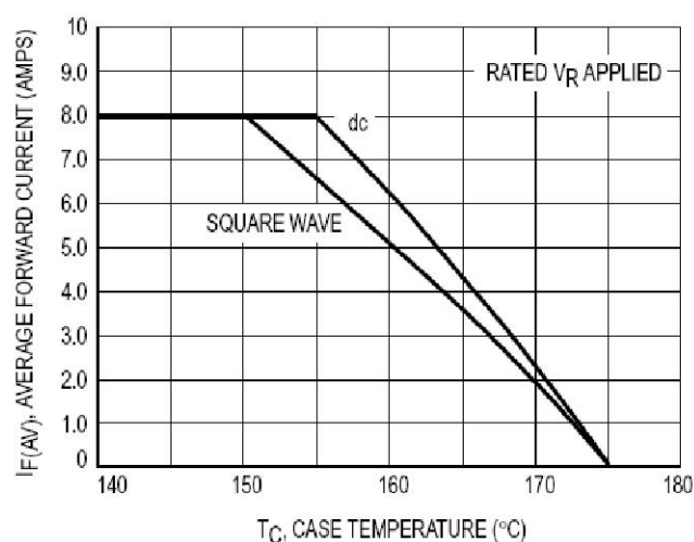
Figure 5. Power Dissipation
