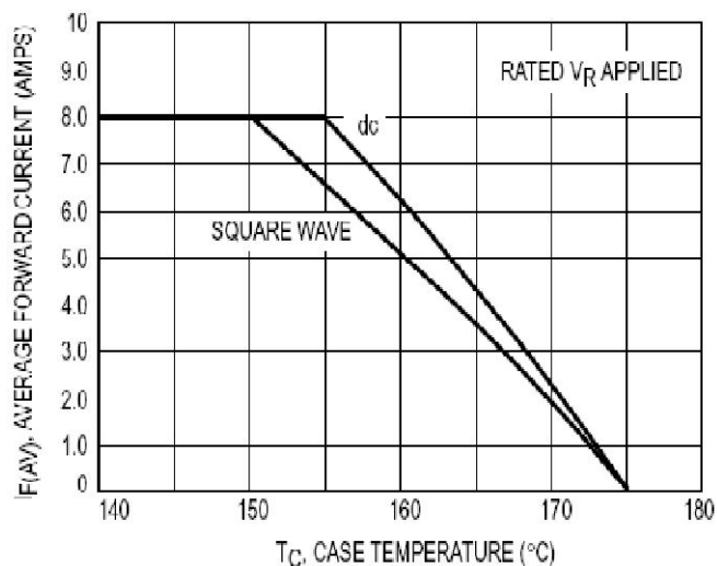
Figure 5. Power Dissipation
