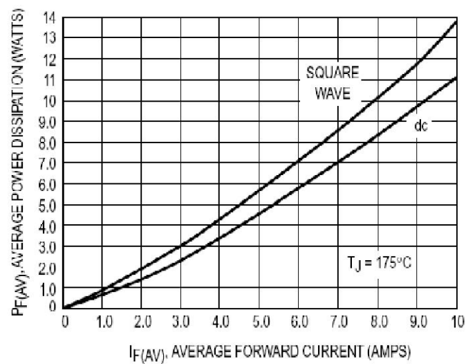
Figure 5. Power Dissipation
