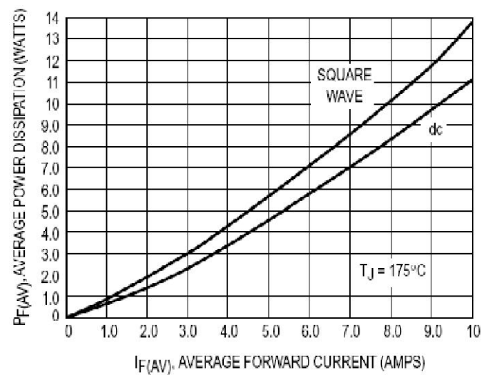
Figure 5. Power Dissipation
