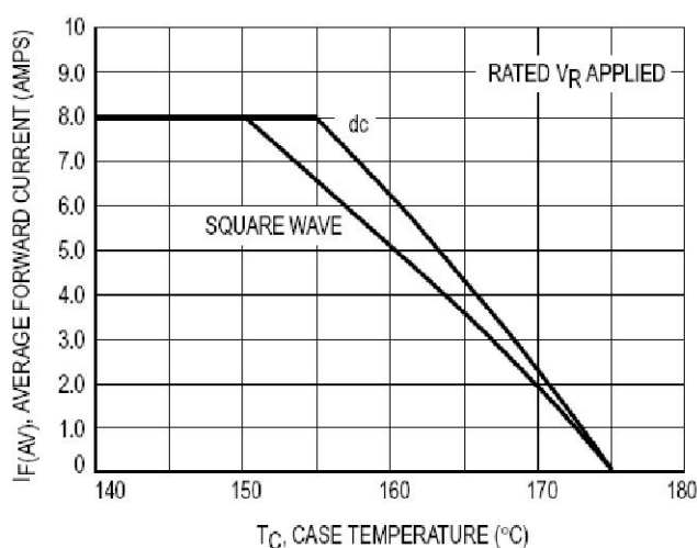
Figure 5. Power Dissipation
