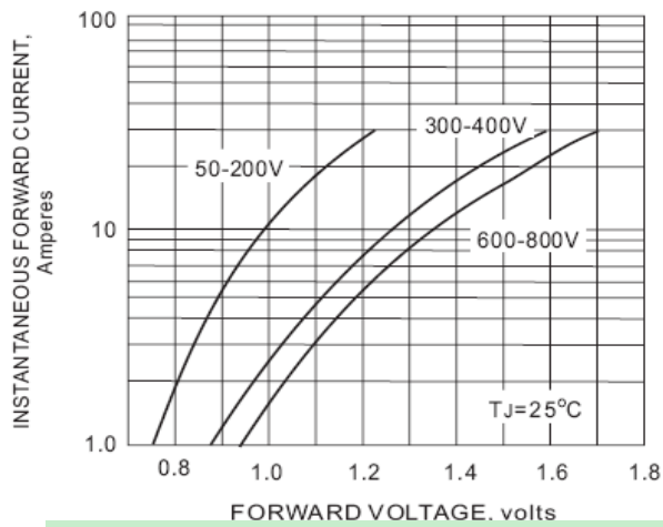
Fig.3 FORWARD CHARACTERISTICS
